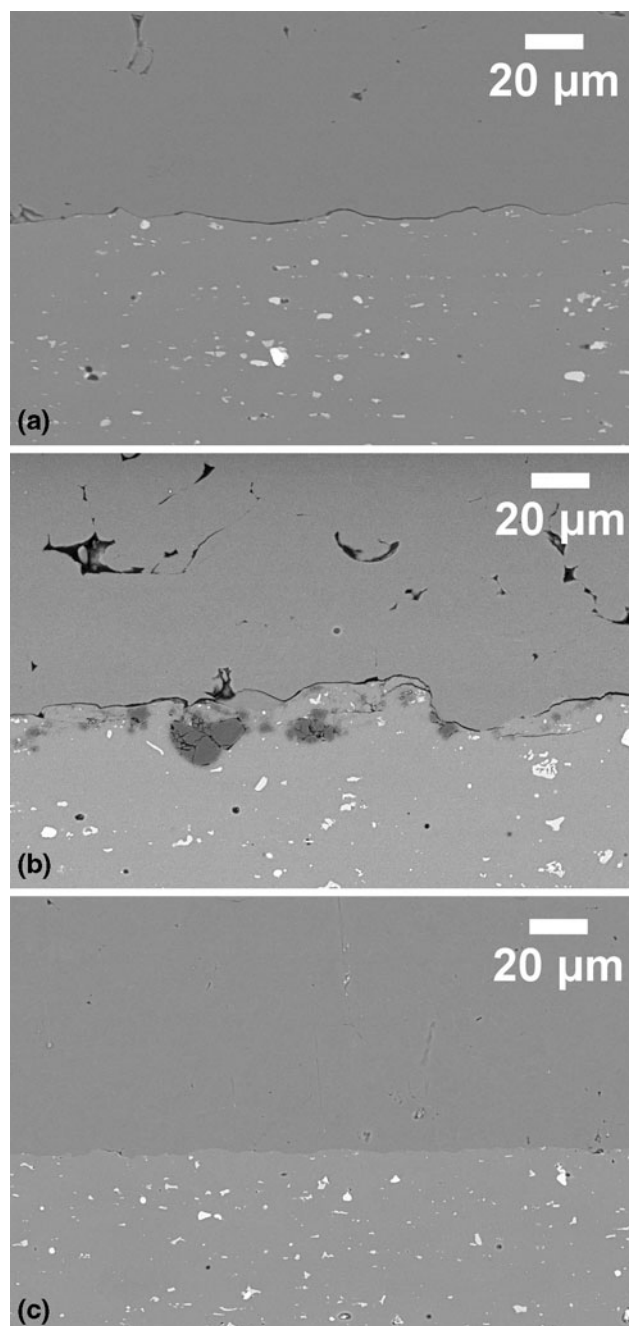
Fig. 6 SEM of cross-sections of cold-sprayed Al coatings formed onto (a) as-received substrate, (b) grit-blasted substrate, (c) laser irradiated substrate ( 2.2 \text{ J} \cdot \text{cm}^{-2} , 150 Hz)
