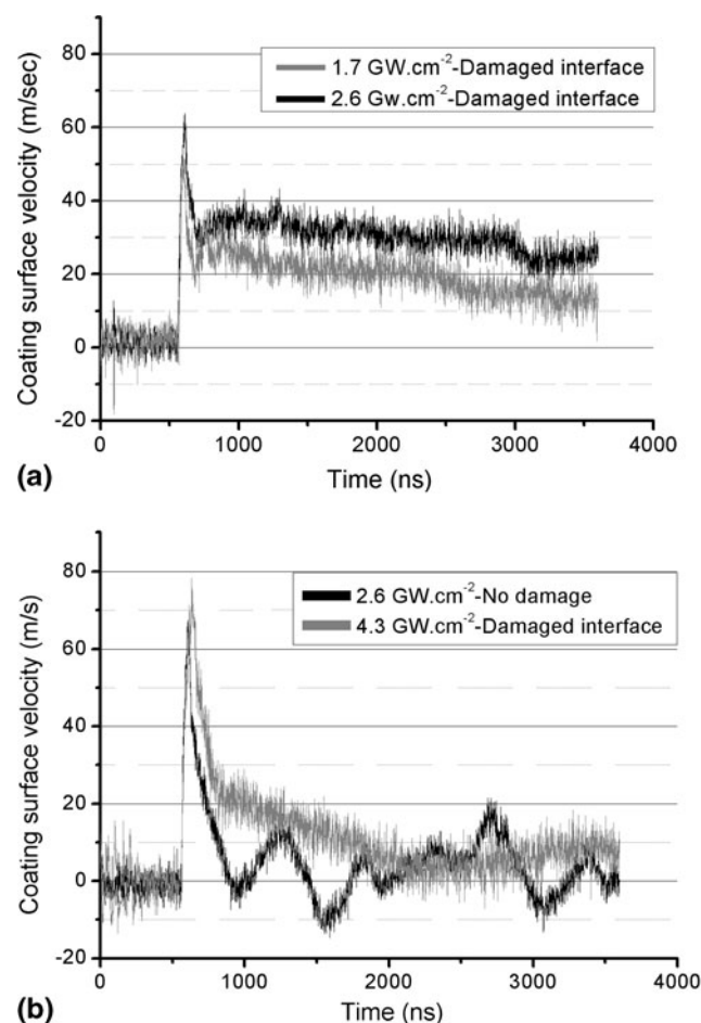
Fig. 10 Velocity profiles of cold-sprayed Al surface on (a) as-received AISI 2017 substrate; (b) laser pre-treated ( 2.2 \text{ J} \cdot \text{cm}^{-2} , 150 Hz) substrate AISI 2017
